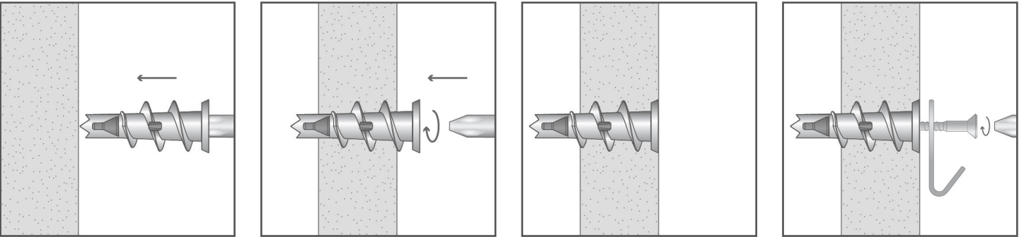
Pierce plasterboard with plug.
